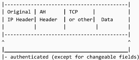
Figure 4: Transport Mode AH packet
