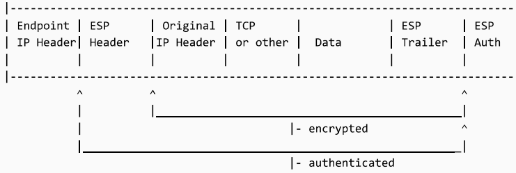
Figure 1: Tunnel Mode ESP packet
