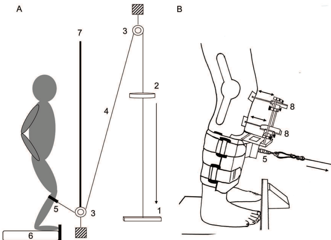
Figure 1. Schematic drawing of the experimental setup. A: Experimental setup, B: Measurement system | 1: stopper, 2: falling weight, 3: pulley, 4: steel rope, 5: force transducer, 6: force plate, 7: visual cover, 8: linear potentiometer. Arrows indicate the direction of the force. Posterior-anterior tibial translation was assessed by two linear potentiometers (8) placed on the patella and the tibial tuberosity. A force transducer (5) was used to measure the force transmitted to the shank.
