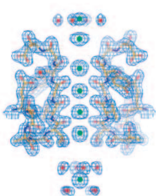
Figure 4. Electron density ( 2F_o - F_c contoured at 2\sigma ) from a high-resolution structure of the KcsA K^+ channel is shown as blue mesh. This region of the channel features the selectivity filter with K^+ ions and water molecules along the ion pathway. The refined atomic model is shown in the electron density. Adapted from (Zhou et al. , 2001b).
