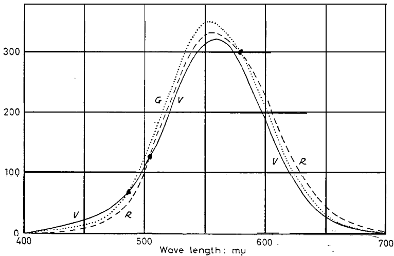
Fig.1. Spectral distribution of the primaries V, G and R, according to the hypothesis of S. Hecht (Bulletin No. 4 of the Howe Laboratory of Ophthalmology, Harvard University Press, Cambridge, Mass., 1931).
