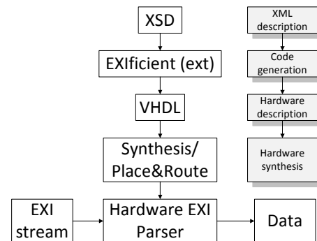
Figure 1: Hardware EXI parser generation
