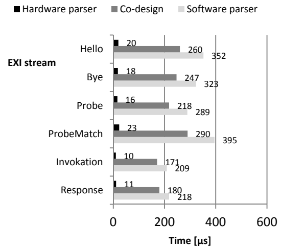
Figure 6: Comparison of processing time of different EXI parser implementations for specific Web service messages
