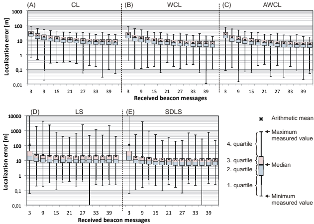
Figure 6. Accuracy of the investigated localization algorithms in the scenario “Dry Tall Underbrush”
