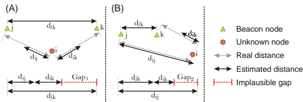
Figure 8. Implausible distance estimations (A) Condition 1, (B) Condition 2. For condition 3, exchange j and k in (B)
