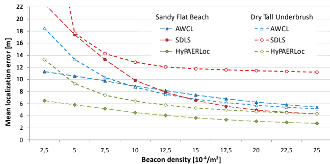
Figure 11. Average mean localization error versus beacon density. Only nodes with at least 3 beacons in range were considered
