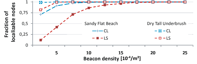
Figure 3. Fraction of localizable nodes versus beacon density. Coarse-grained algorithms require at least 1 received beacon, fine-grained algorithms at least 3 received beacons
