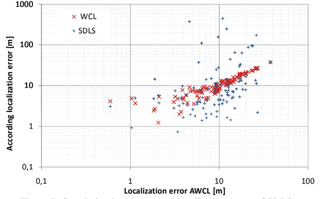
Figure 7. Correlation between sorted localization errors of SDLS-measurements and according localization errors of AWCL
