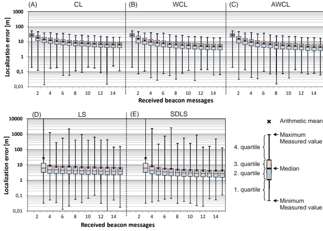
Figure 5. Accuracy of the investigated localization algorithms in the scenario “Sandy Flat Beach”
