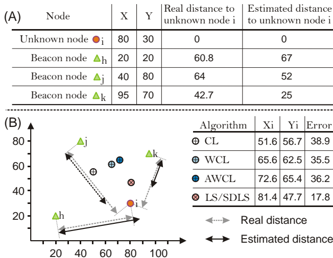
Figure 1. Example Localization (A) Example setup with erroneous distance estimations, (B) Visualization and results. All values in meters.
