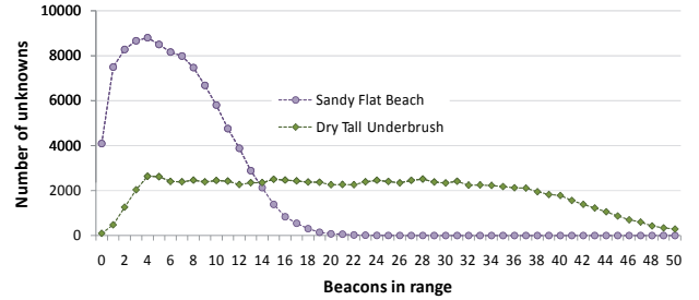
Figure 4. Overall number of simulated unknowns with certain beacons in range
