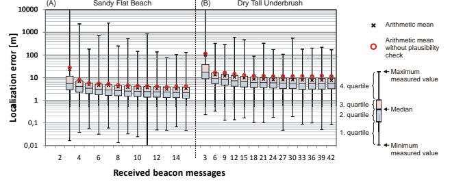
Figure 9. Accuracy of SDLS with plausibility check in both investigated scenarios
