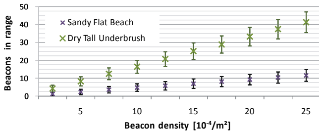
Figure 2. Beacons in range versus beacon density
