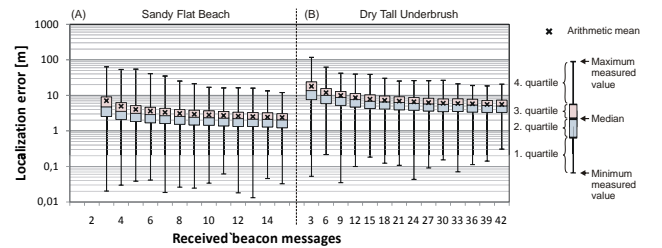
Figure 10. Accuracy of HyPAERLoc in both investigated scenarios
