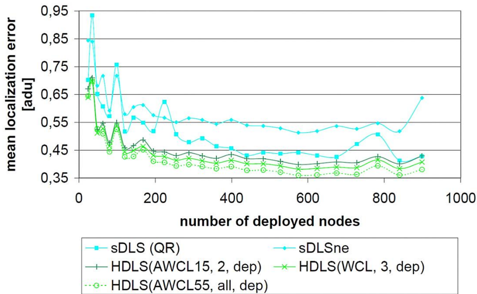
Fig. 17. Mean localization error of best performing HDLS approaches for different limits of virtual beacon nodes.
