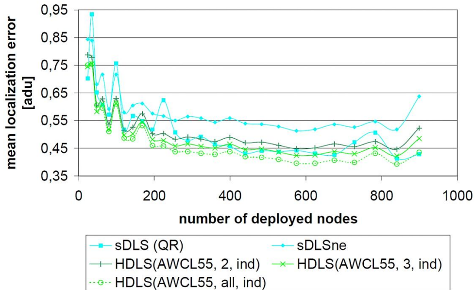
Fig. 10. Mean localization error of AWCL based HDLS with independent distance estimation.
