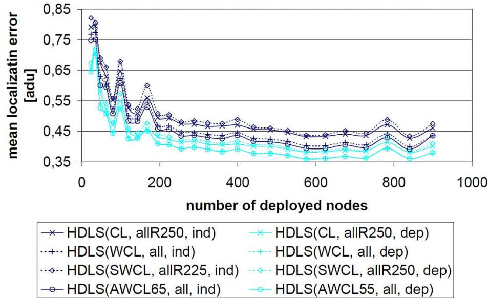
Fig. 16. Mean localization error of best performing HDLS approaches, grouped by estimation technique and distance approximation.
