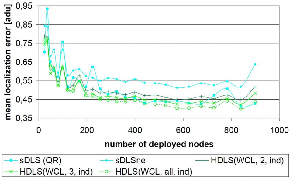
Fig. 8. Mean localization error of WCL based HDLS with independent distance estimation.
