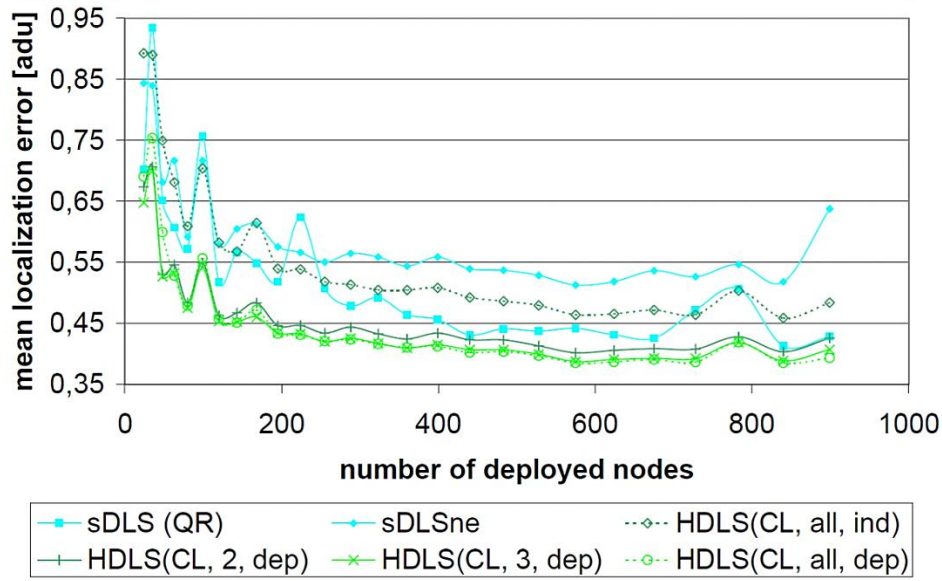
Fig. 15. Mean localization error of CL based HDLS with dependent distance estimation.
