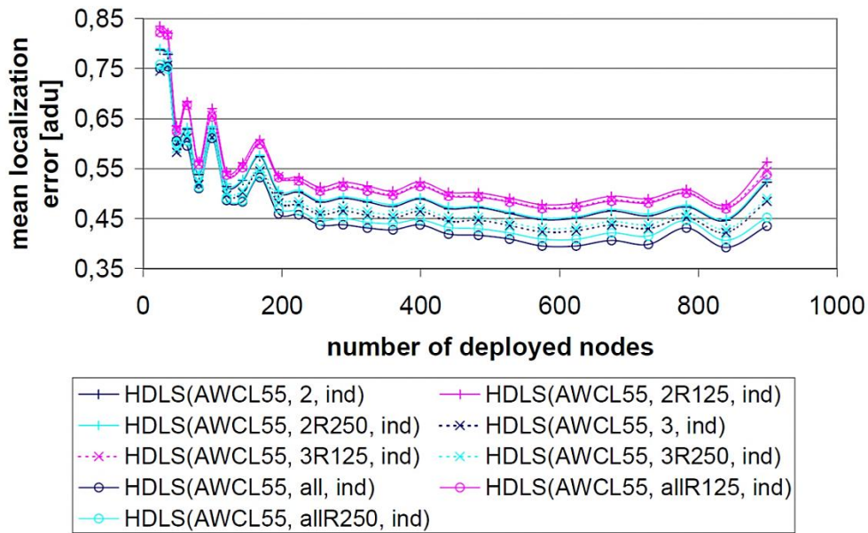
Fig. 12. Mean localization error of AWCL based HDLS with independent distance estimation and range based virtual beacon strategy.
