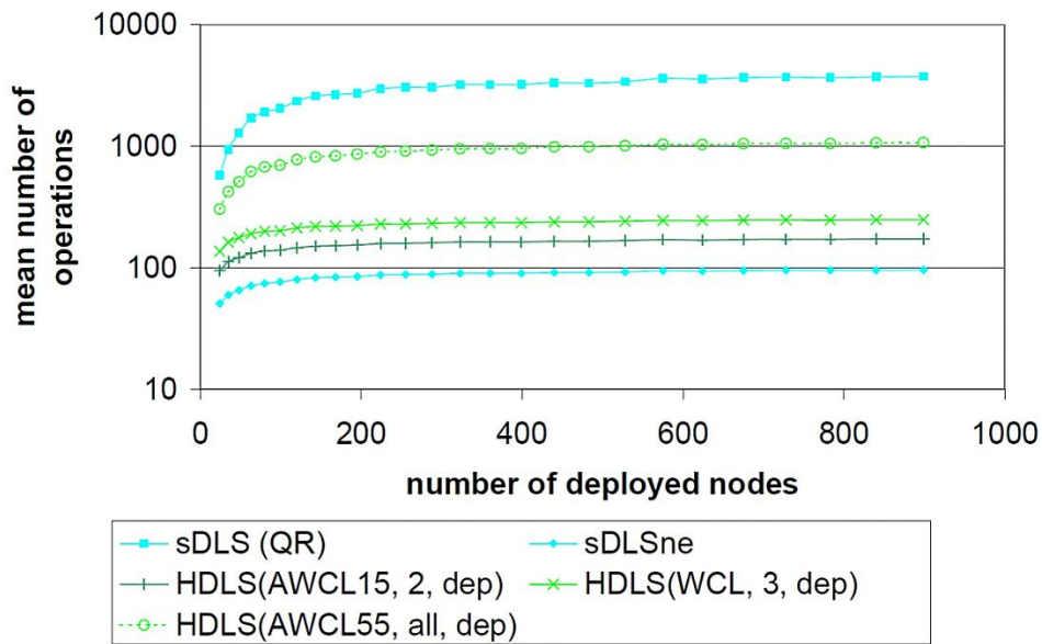
Fig. 19. Mean number of operations of best performing HDLS approaches for different limits of virtual beacon nodes.
