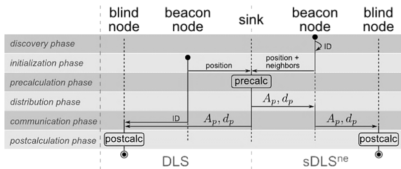
Fig. 1. Algorithmic comparison of DLS and sDLS ne .
