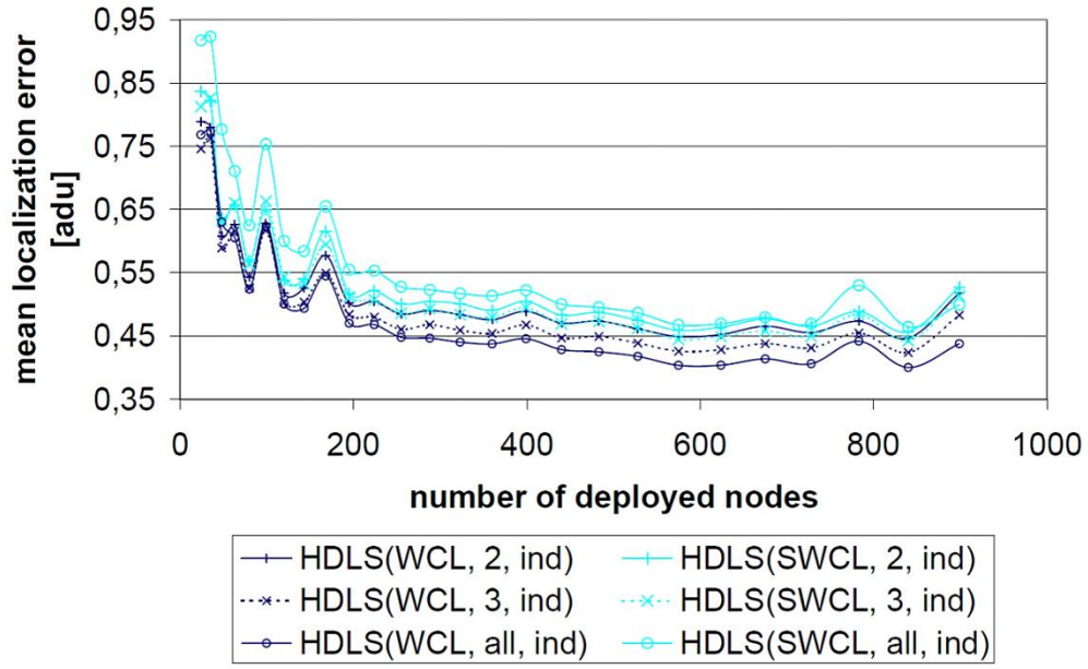
Fig. 9. Mean localization error of HDLS based on WCL and SWCL with independent distance estimation.
