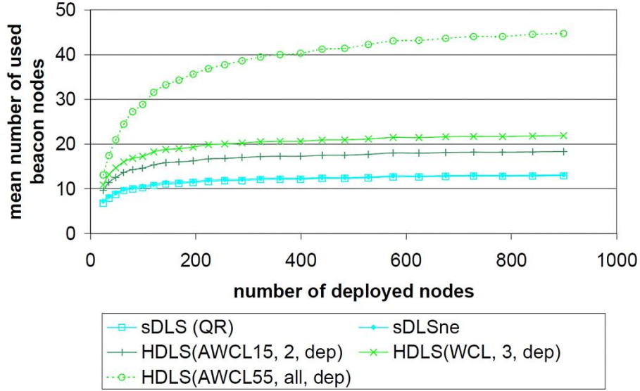
Fig. 18. Mean number of used beacon nodes of best performing HDLS approaches for different limits of virtual beacon nodes.
