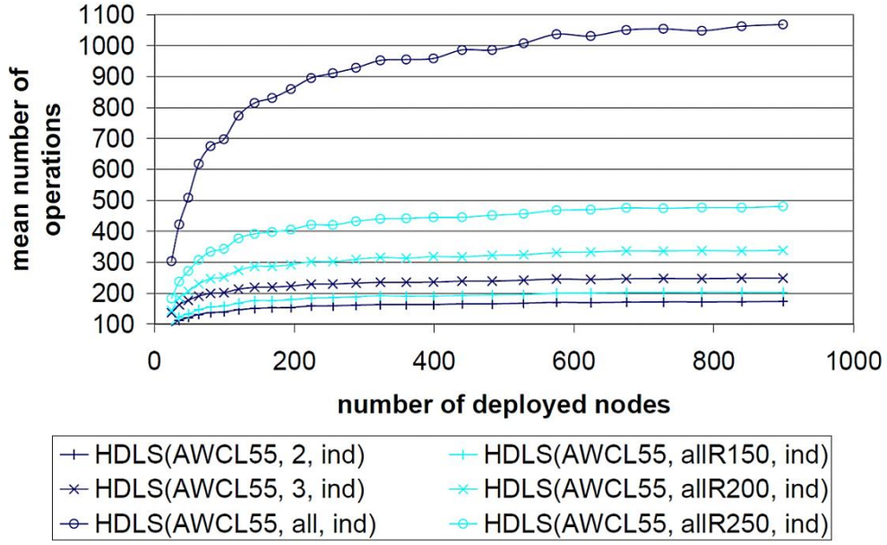
Fig. 14. Range based equivalents of AWCL based HDLS approaches with independent distance estimation – mean number of operations.
