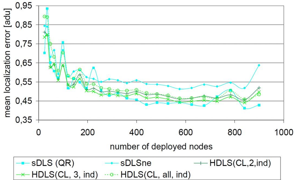
Fig. 7. Mean localization error of CL based HDLS with independent distance estimation.
