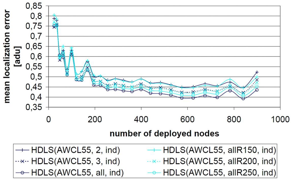
Fig. 13. Range based equivalents of AWCL based HDLS approaches with independent distance estimation – mean localization error.
