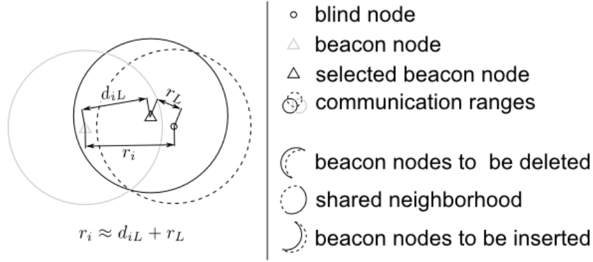
Fig. 3. Approximation of a distance between blind node and inaccessible beacon node i by means of the linearizing beacon node L .
