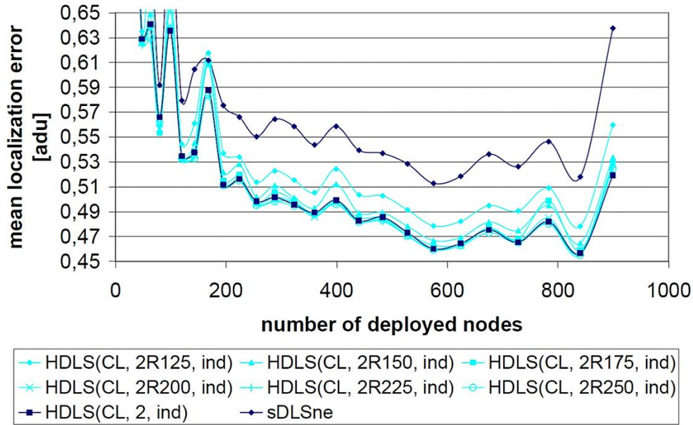
Fig. 11. Mean localization error of CL based HDLS with independent distance estimation and range based virtual beacon strategy.
